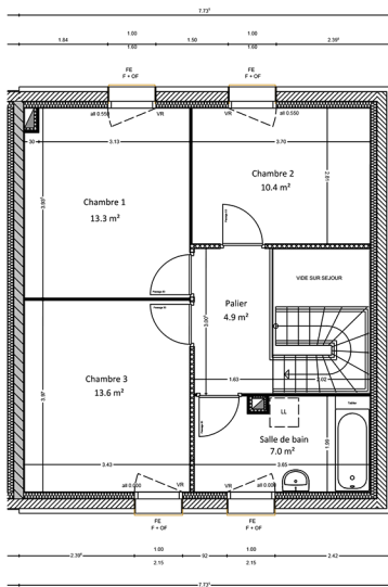
PLAN R+1
